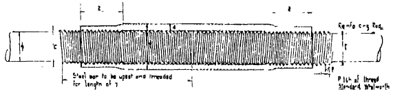
HALF FULL SIZE DETAIL OF SCREW COUPLING.
